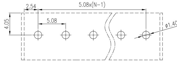
PCB LAYOUT
